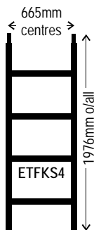
4 RUNG S/W FRAME Weight: 5.0kg
