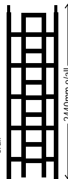
ETFSL5 5 RUNG S/W LADDERFRAME Weight: 13.0kg
