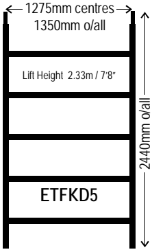
5 RUNG D/W FRAME Weight: 9.0kg
