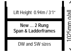
2 RUNG D/W FRAME Weight: 4.0kg
